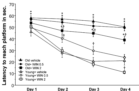
Fig. 1. Water maze performance. During days 2 and 3, young rats receiving the 0.5 mg/kg WIN dose (open circle) performed significantly worse than rats in the other two young groups (open triangle and open square) ( ^{\dagger}p < 0.05 ). On day 4, the young rats receiving the 2 mg/kg WIN dose (open square) performed significantly better than the other two groups of young rats (open triangle and circle, ^{\ddagger}p < 0.05 ). Old rats were significantly impaired as compared to young rats ( ^{\ast}p < 0.05 ). WIN-55212-2 2 mg/kg (closed square) improved performance of age rats (closed triangle, ^{\ddagger}p < 0.05 ).
